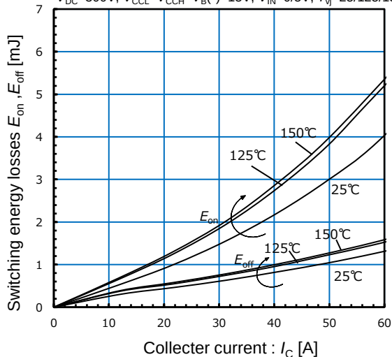
Typical switching loss vs. Collector current
