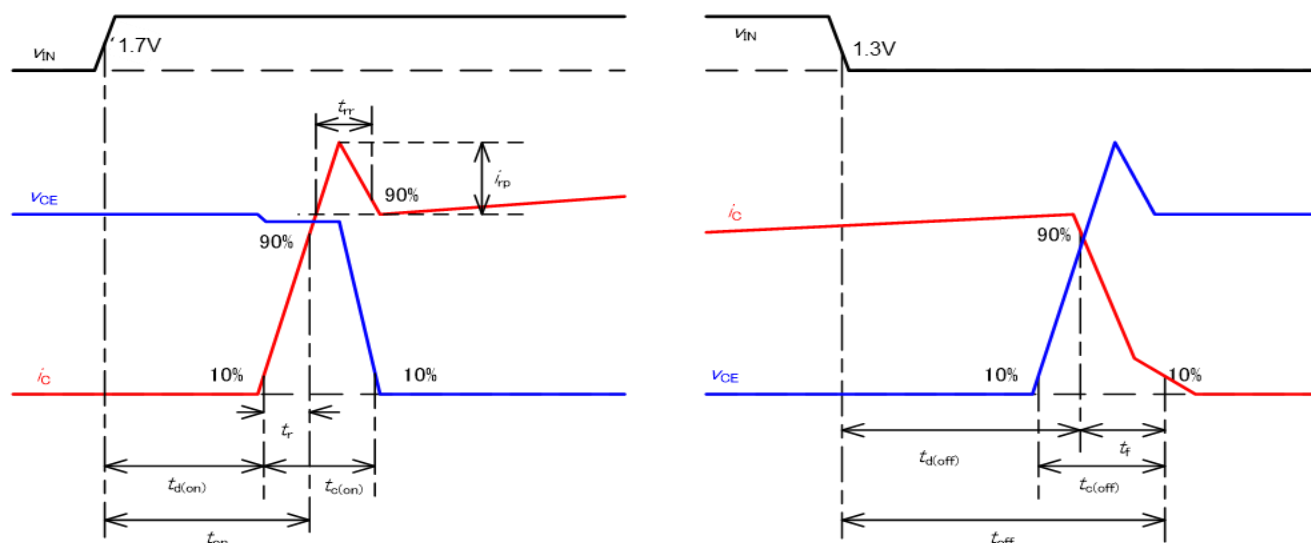
Fig.2-1 Switching waveforms
