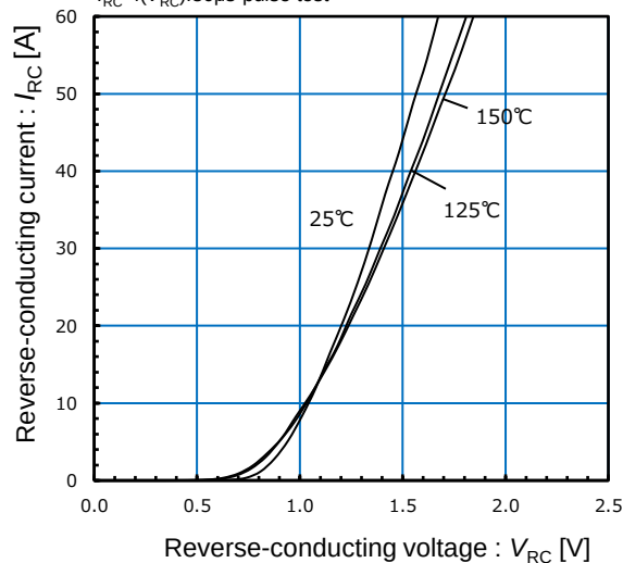
Typical reverse-conducting voltage characteristics
