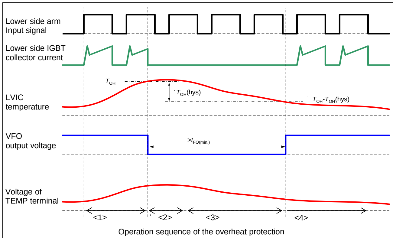
Fig.2-6 Overheat protection
