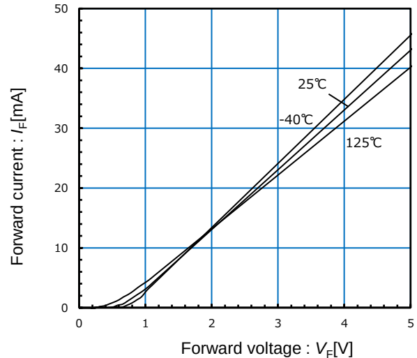
Zoom up typical BSD forward voltage drop characteristics
