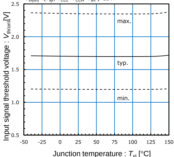
Input signal V_{th(on)} characteristics
