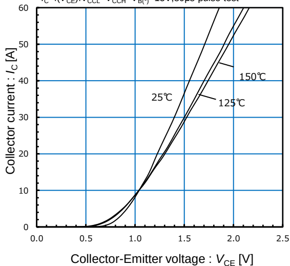
Typical on-state voltage drop characteristics
