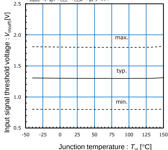
Input signal V_{th(off)} characteristics
