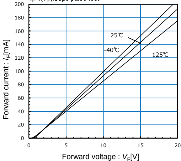
Typical BSD forward voltage drop characteristics
