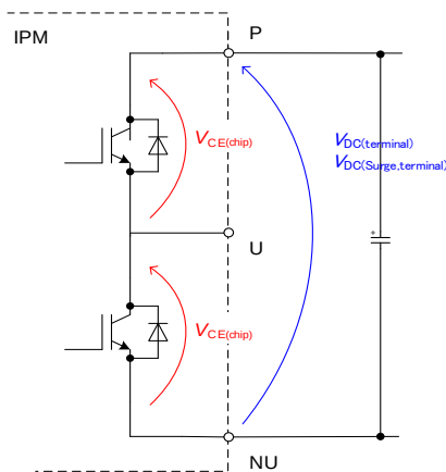
Fig.2-2 Rated Voltage
